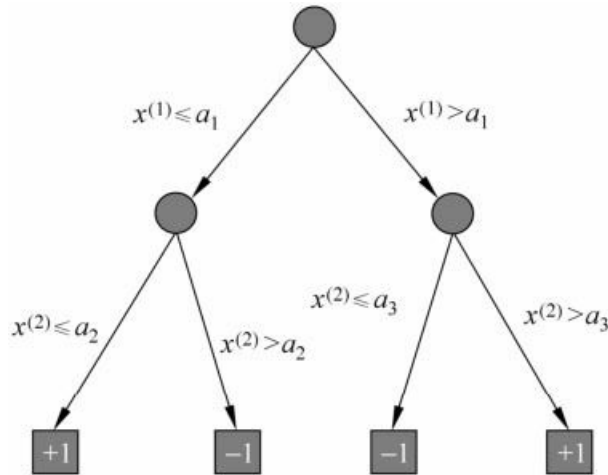
(c) 决策树
